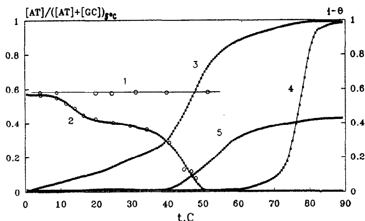
Fig. 2. The temperature dependence of the AT pairs fraction \{[AT]/([AT] + [GC])_{5^{\circ}\text{C}}\} of the AF-40-nucleotide complexes (left ordinate). 1 = anti-parallel duplex IV-V; 2 = parallel duplex IV-VI. 3,4 (right ordinate) = thermal denaturation curves (1-\theta) of parallel IV-VI and antiparallel - IV-V 40-duplex, respectively. 5 = the melting curve of GC pairs calculated by subtraction from the curve (3) of the contribution of melted AT pairs estimated with the help of curve (2). Oligonucleotide concentration was 2.4 \times 10^{-4} M(N); 0.01 M phosphate buffer, pH 7, 0.25 M NaCl; AF concentration was 10^{-6} M. [AT]/([AT] + [GC])_{5^{\circ}\text{C}} = \theta(q/q_{AT})^{1/2} , where [AT] is the AT pair concentration in the 40-nucleotide studied in dependence on temperature, ([AT] + [GC])_{5^{\circ}\text{C}} is the total base pairs concentration at 5^{\circ}\text{C} in the 40-nucleotide [7].
